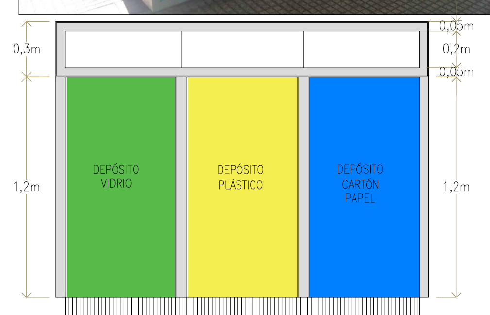
VISTA FRONTAL
